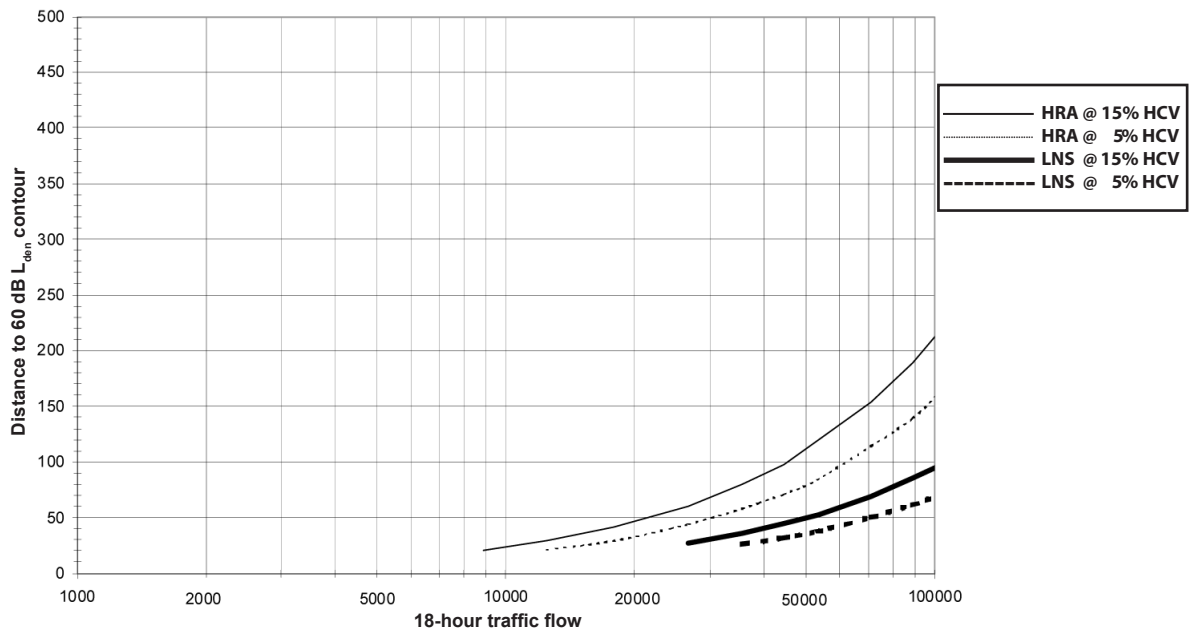
Road in False Cut, Receiver 1.5 m AGL, 100km/h traffic speed
